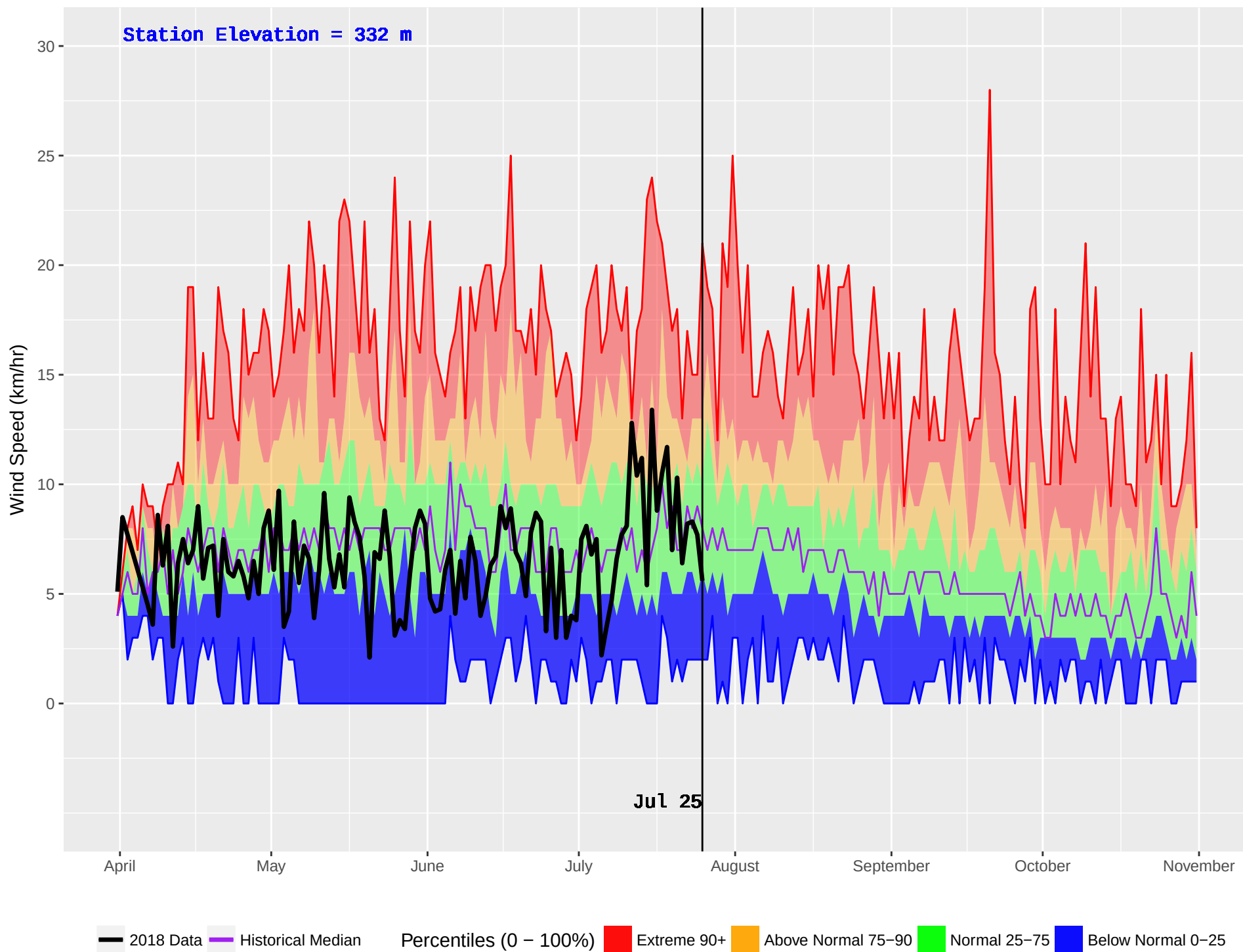
MACHMELL (101) : Historical (1990–2016) and Current (2018) Noon Wind Speed
